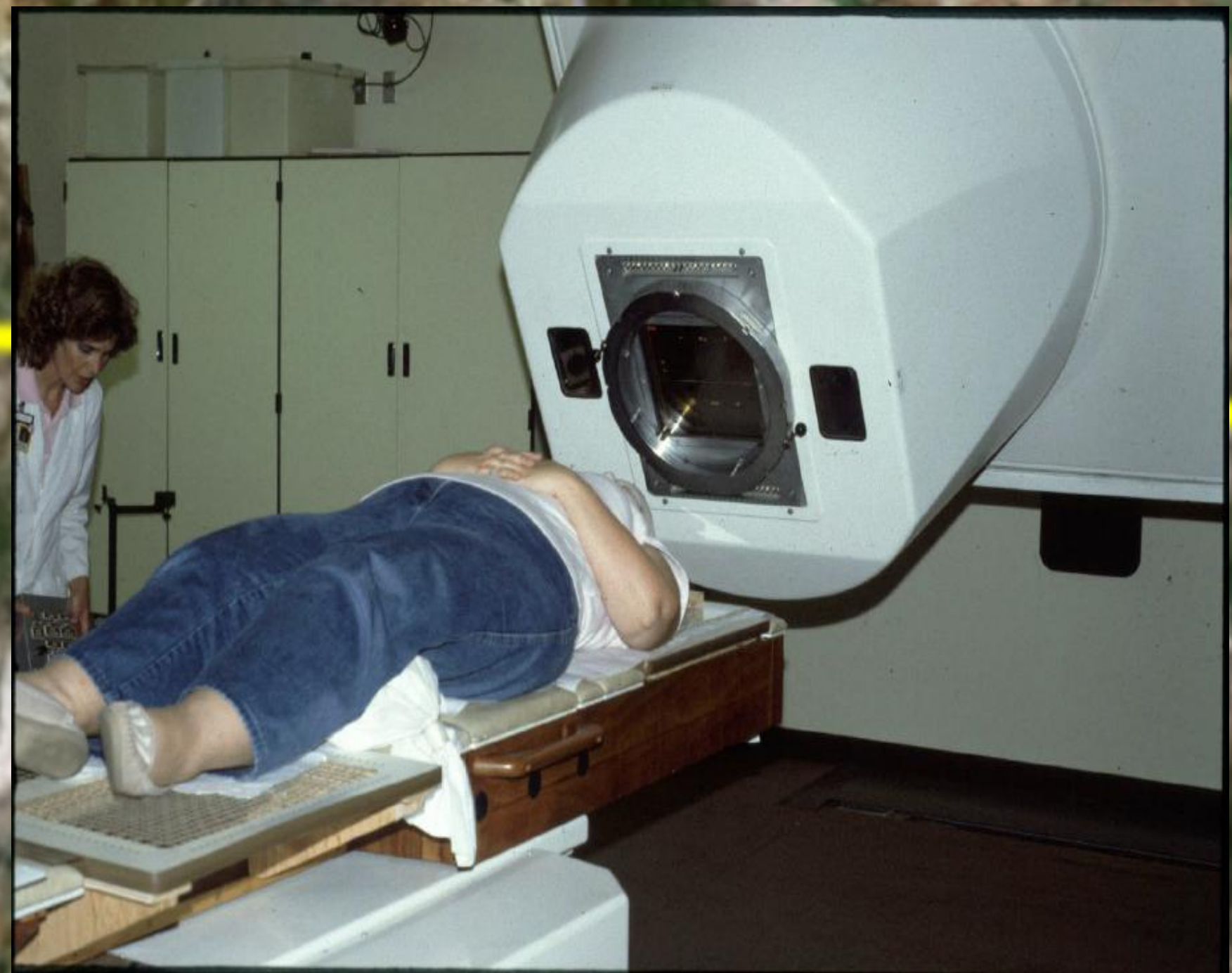
Neutrons
